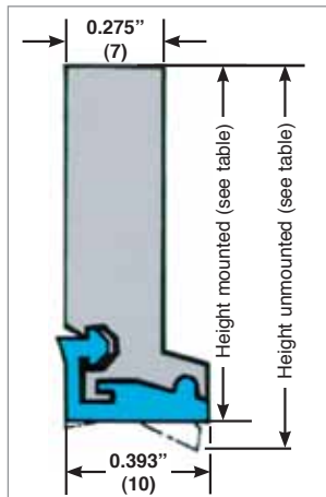
TYPE BAS Thicker aluminum profile with lip for mounting optional hot-chip shield.
